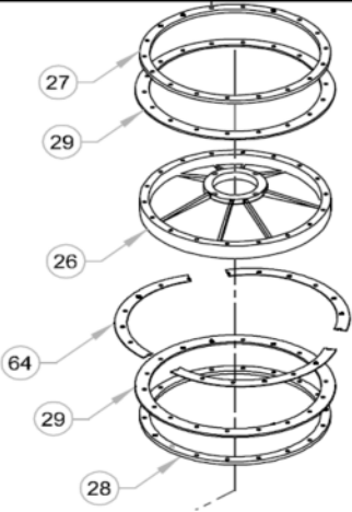
Figure 3. Piston Seals
